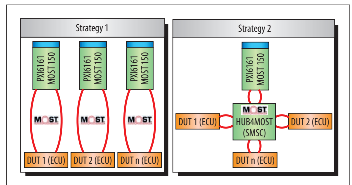
Figure 3. MOST PXI test system strategies.
