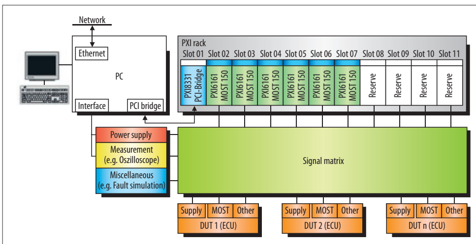
Figure 1. Architecture test system.
